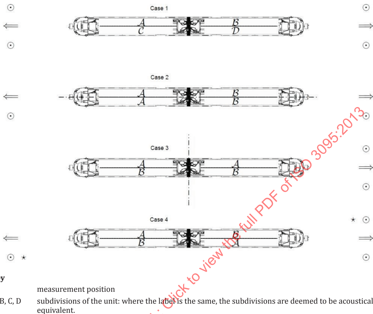
Figure 11 — Measurement positions for different cases of unit layout symmetries
