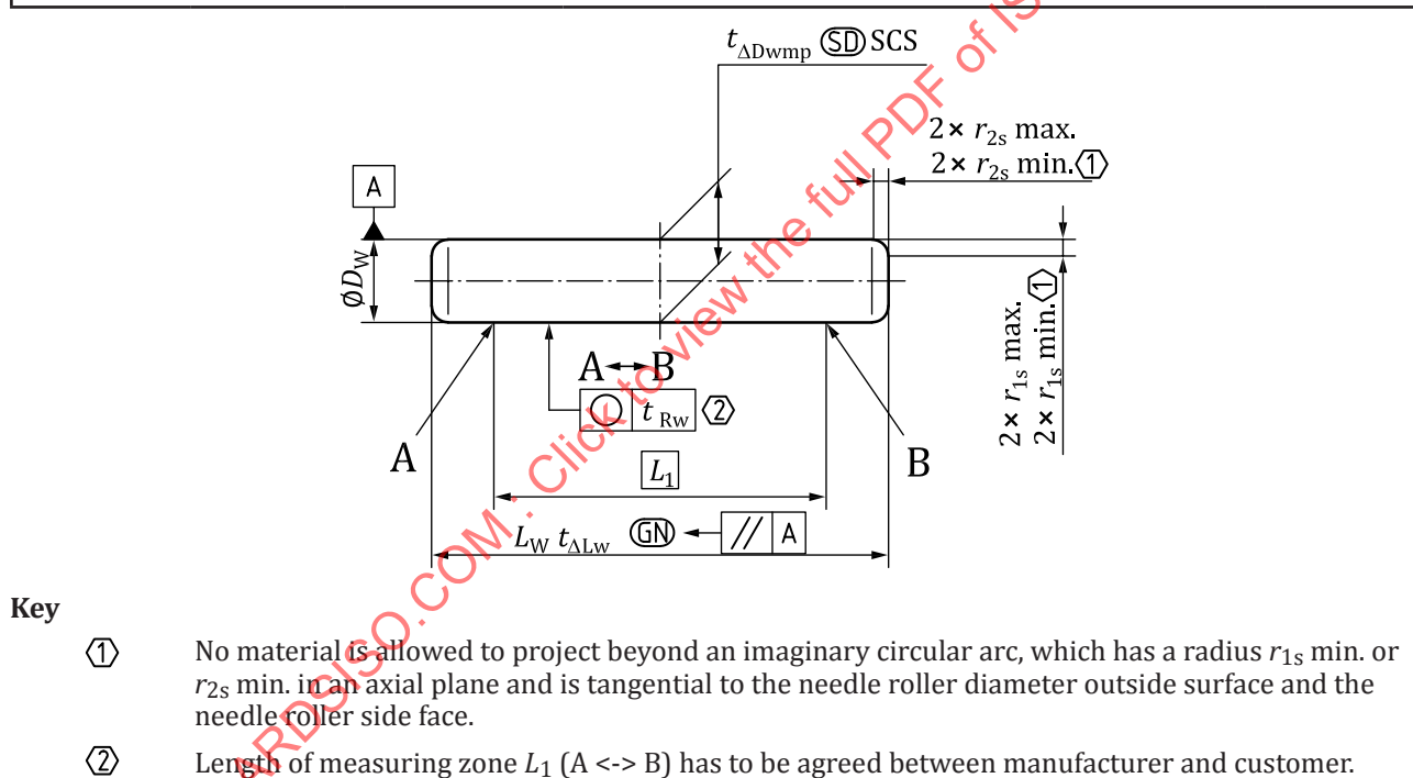
Figure 1 — Needle roller with flat ends
