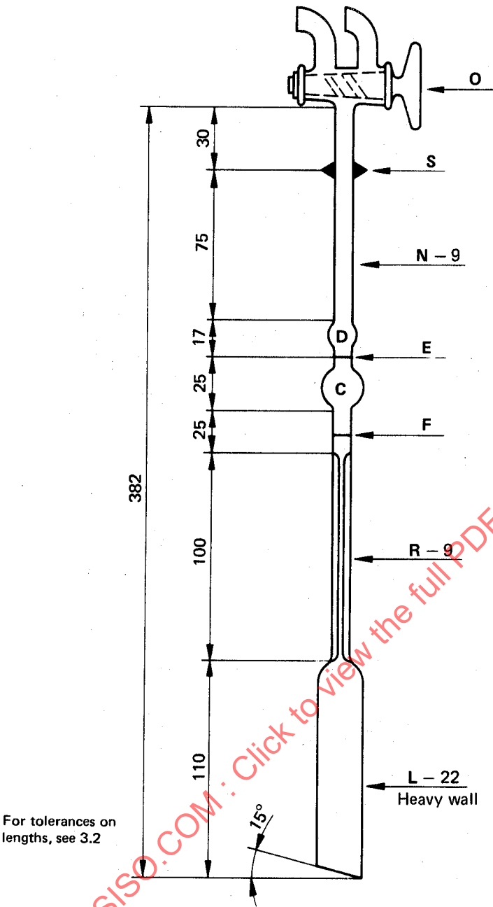
FIGURE 13 — Atlantic viscometer
