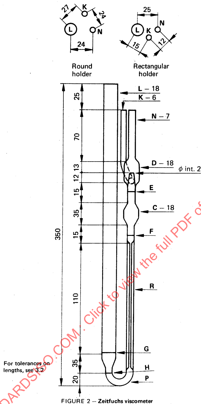
FIGURE 2 — Zeitfuchs viscometer
