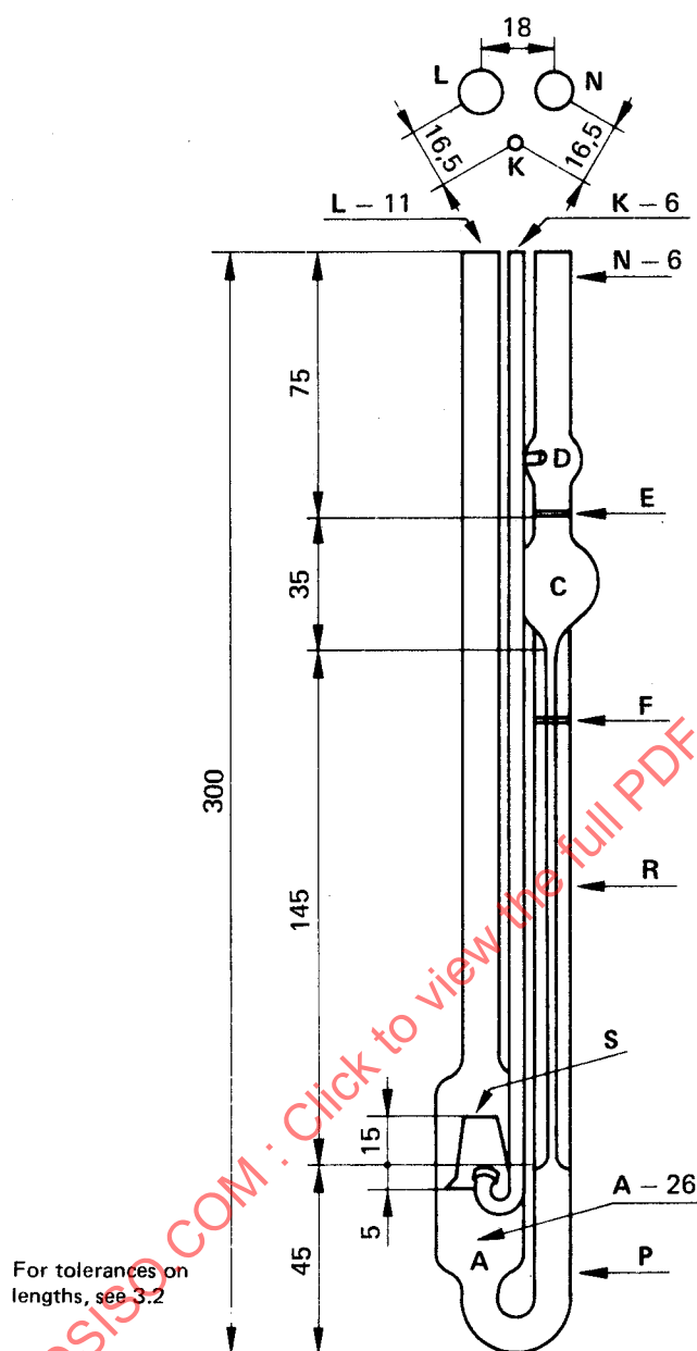
FIGURE 5 – SIL viscometer
