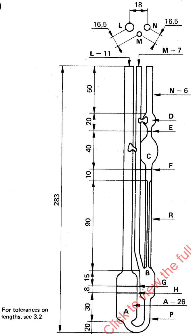
FIGURE 11 – Ubbelohde viscometer
