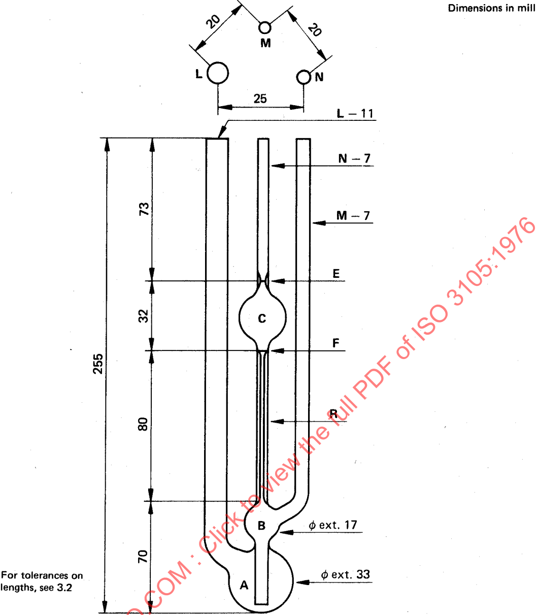
FIGURE 9 – BS/IP/SL(S) viscometer
