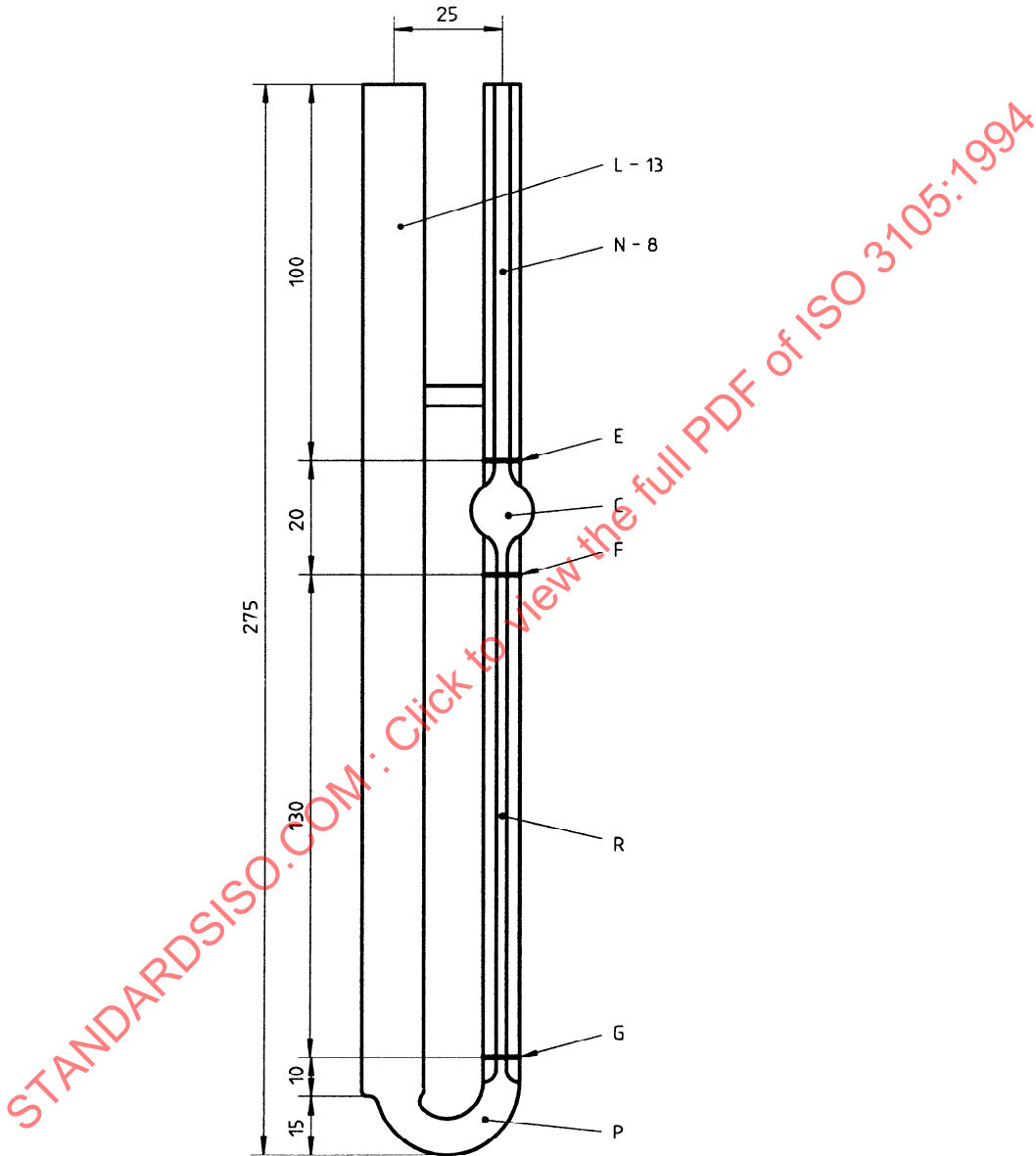
Figure A.6 — Cannon-Manning semimicro viscometer
