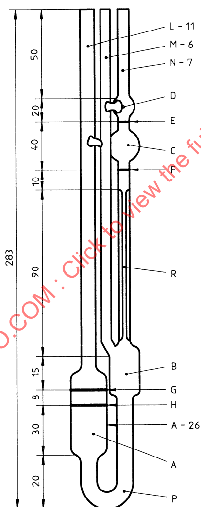
Figure B.4 — Ubbelohde viscometer
