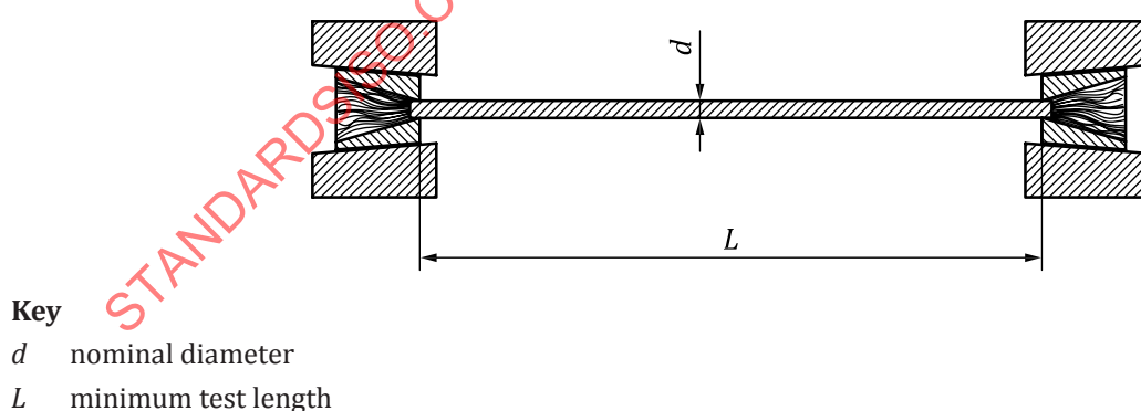
Figure 1 — Test piece terminated by molten metal or resin socketing method.
