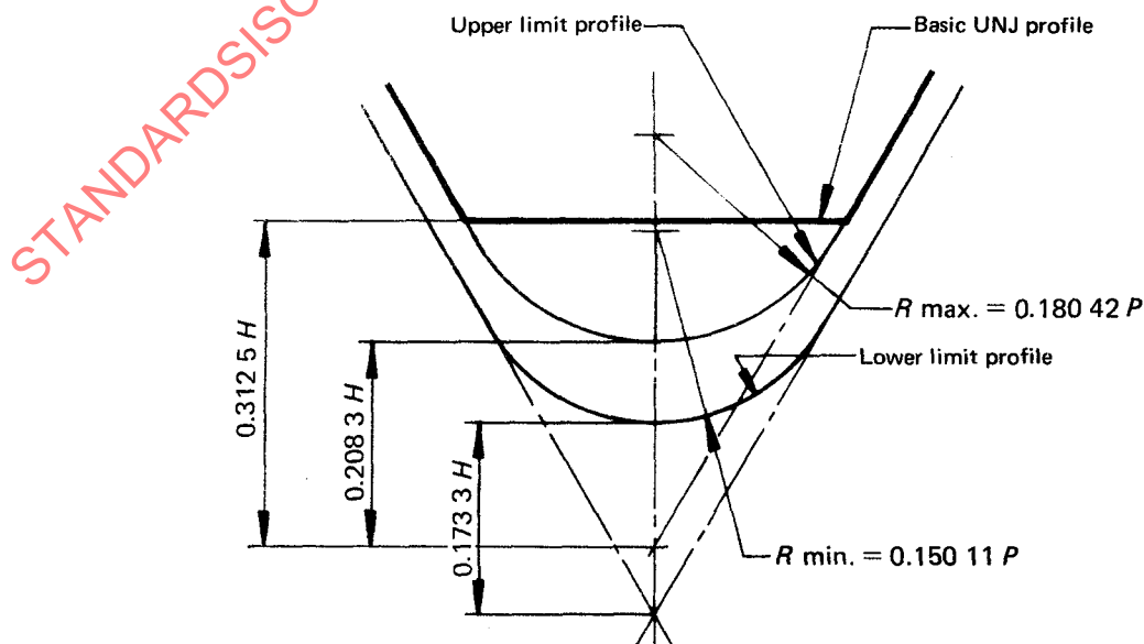
FIGURE 5 — Radius at the root of the screw thread
