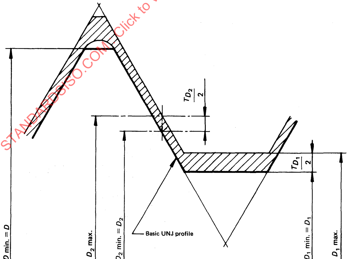
FIGURE 3 — Internal thread tolerances
