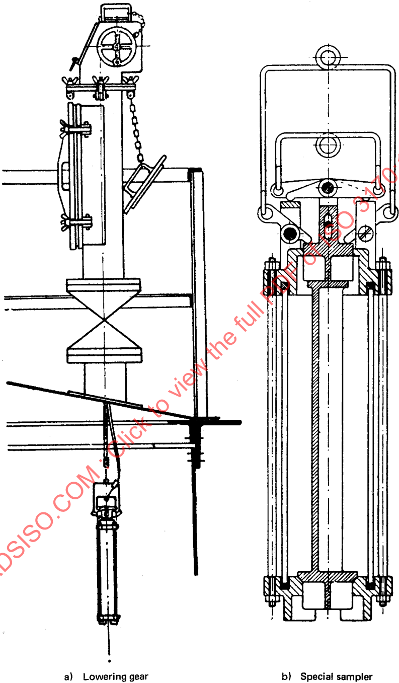
FIGURE 5 — Example of vapour-lock device
