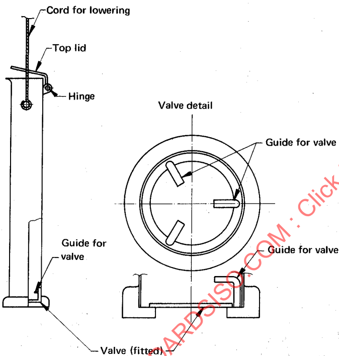
FIGURE 9 — Example of cylinder sampler
