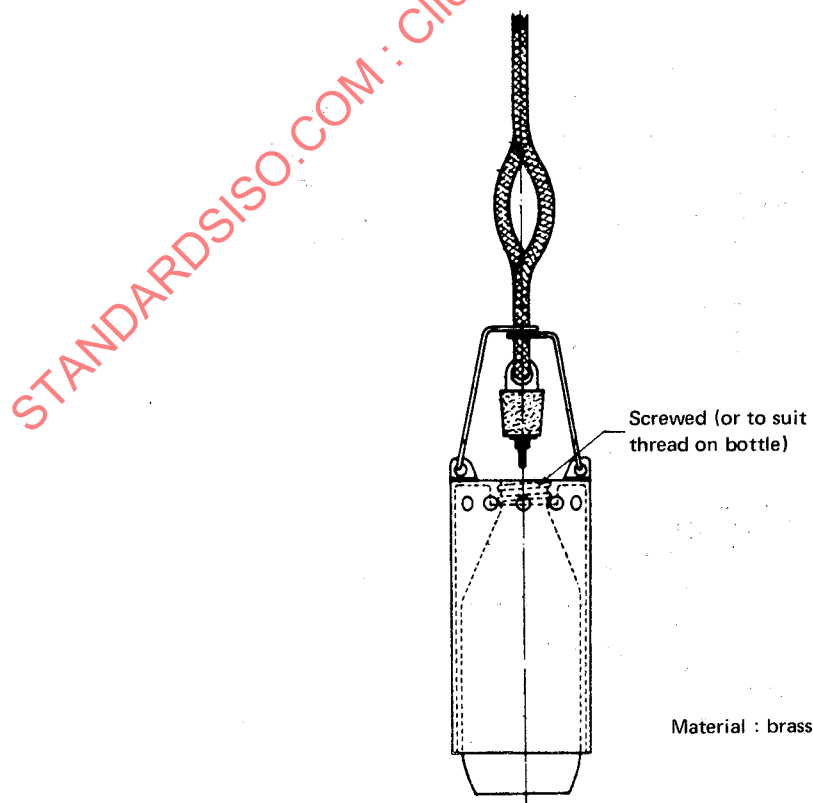
FIGURE 3 — Example of sampling cage for use with screw-top glass 600 ml sample bottle
