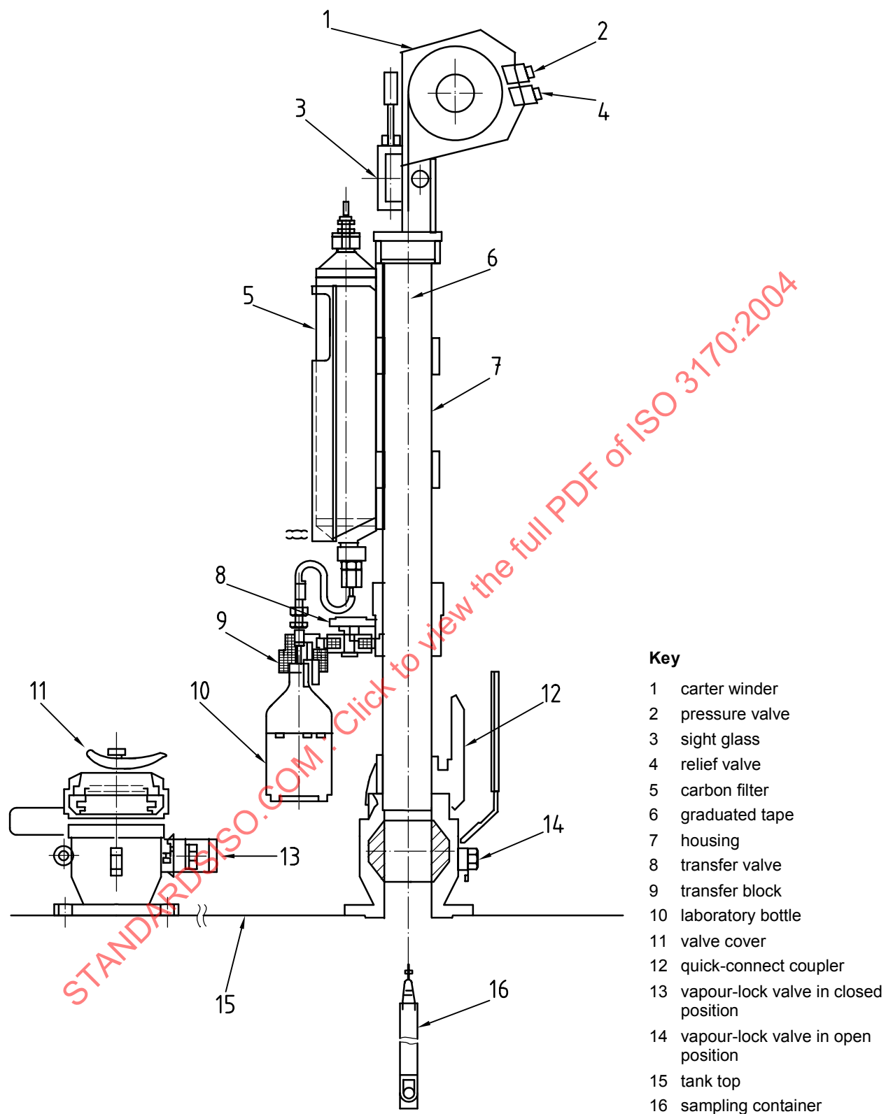
Figure 10 — Example of a lock valve and closed system sampler
