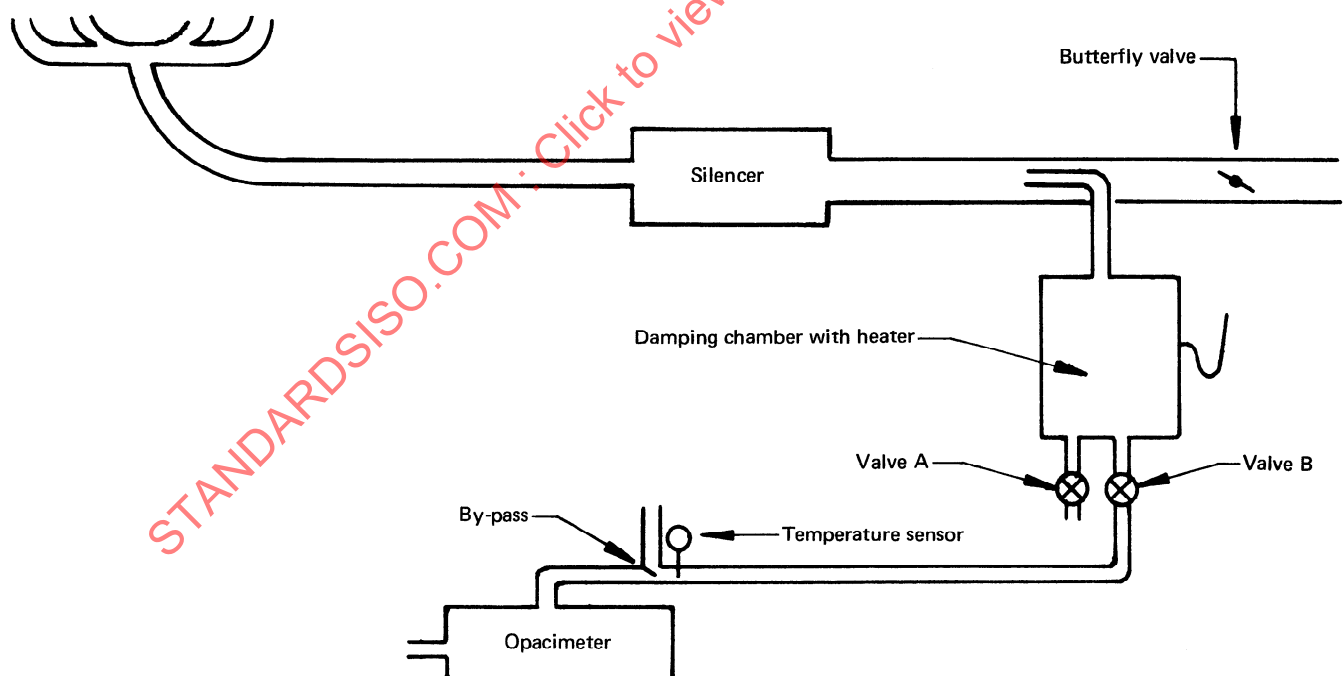
FIGURE 2 — Test installation
