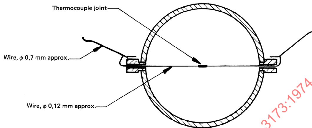
FIGURE 1 — Diametral thermocouple
