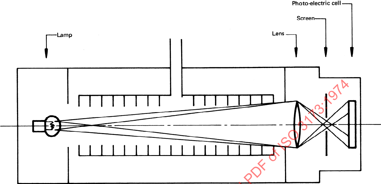
FIGURE 3 – Opacimeter
