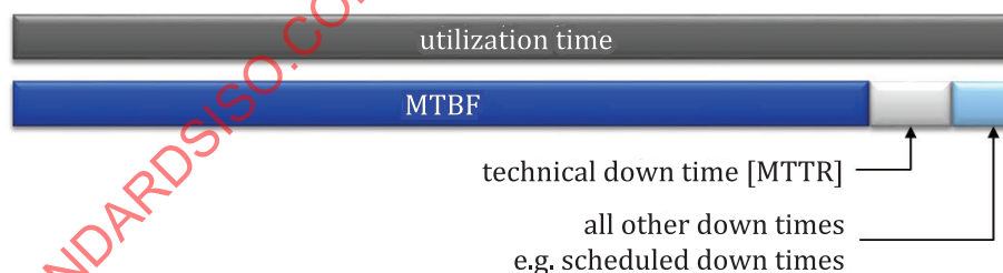
Figure 3 — MTBF as a component of utilization time
