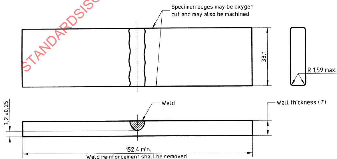
Figure B.2 - Transverse guided-bend test specimen
