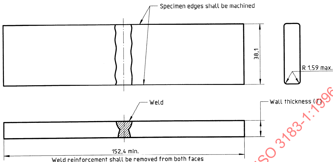
Figure B.1 – Transverse tensile test specimen
