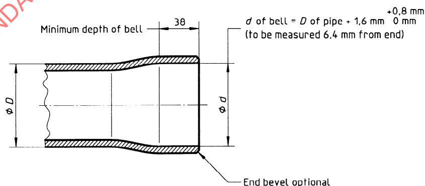
Figure 2 – Belled end for bell and spigot joint
