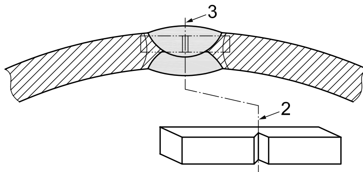
b) Weld specimen
