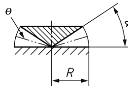
b) Vertical section through measuring gap
