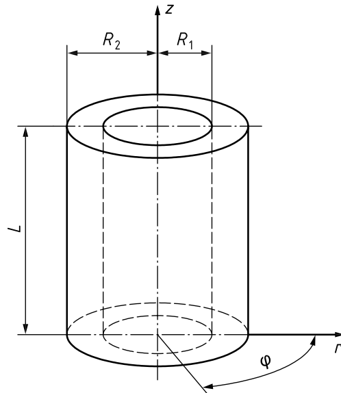
a) Cylindrical coordinates and relevant dimensions
