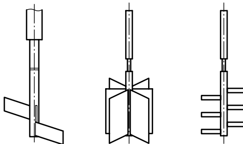
c) Rotors (paddle spindle as per ASTM D562 [2] ), vane rotors and pin rotors
