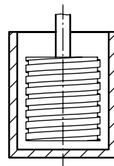
b) Cylinder with a helical spiral groove on the measuring bob (to prevent sedimentation)
