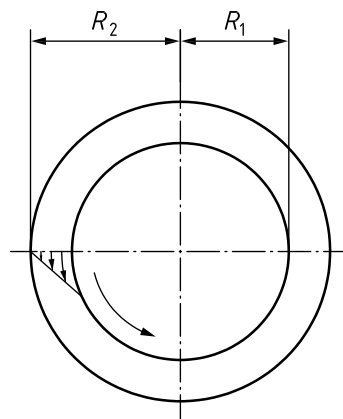
b) Velocity profile and cross-section through the measuring gap perpendicular to the axis of rotation for Couette type
