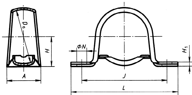
Figure 4 — Pressed plumber block housings
