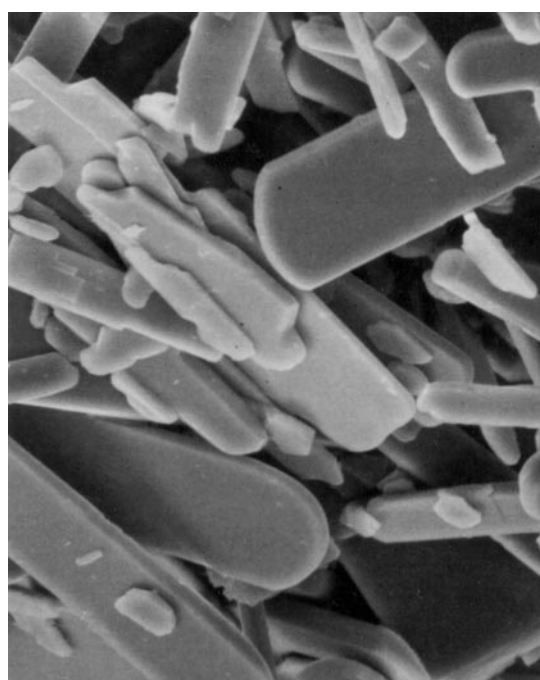
Figure 6 — Flaky (1406) Figure 6 — Lamellaire (1406) Bild 6 — Flittriges Pulver (1406)
