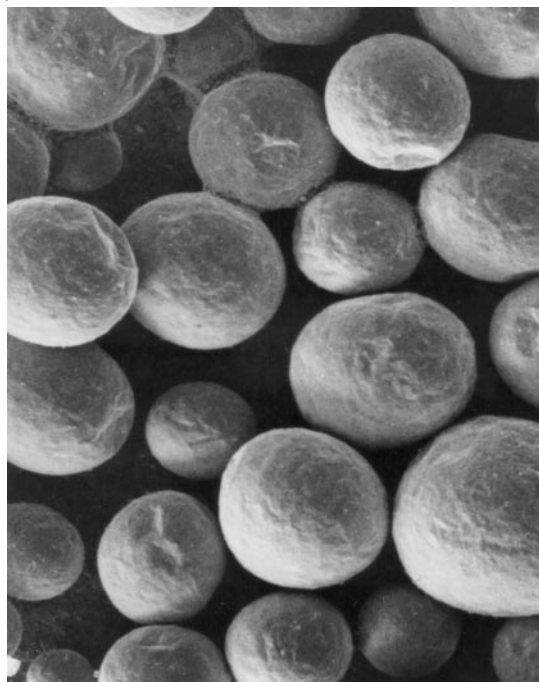
Figure 10 — Spheroidal (1410) Figure 10 — Sphéroidal (1410) Bild 10 — Kugeliges Pulver (1410)
