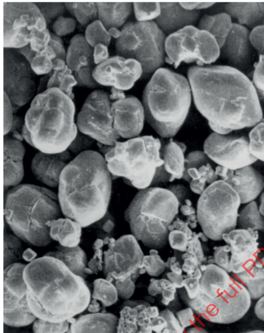
Figure 9 — Nodular
