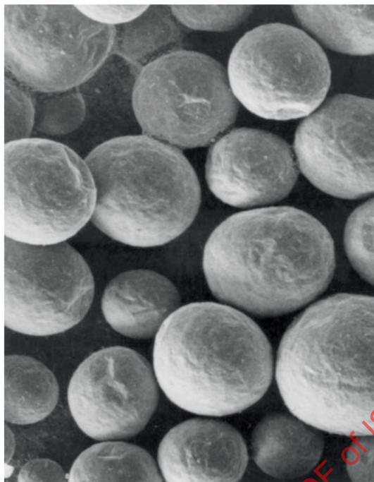
Figure 10 — Spheroidal
