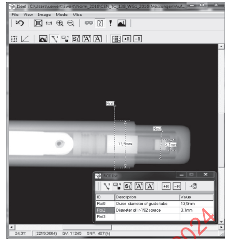
b) Digital image of an Ir-192 gamma radiation source and profile positions at source and guide tube
