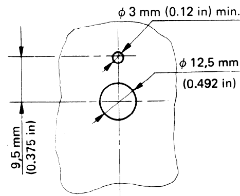
FIGURE 1a) – Panel drilling
