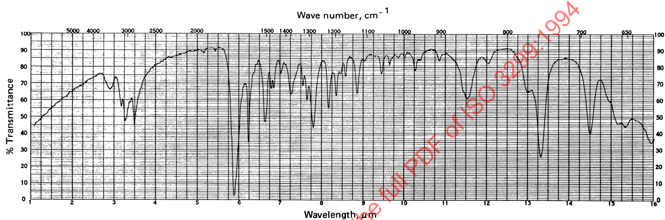
Figure 1 — Reference infrared spectrum of 1-phenyl-3-pyrazolidinone (KBr plate)
