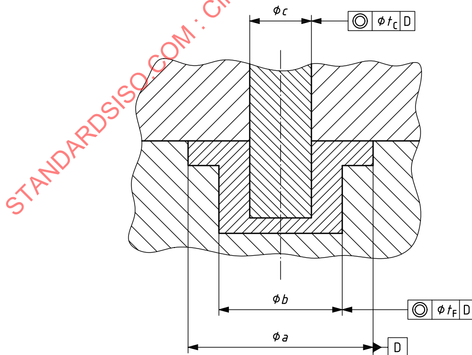
Figure 5 — Example of coaxiality tolerances for a moulded product
