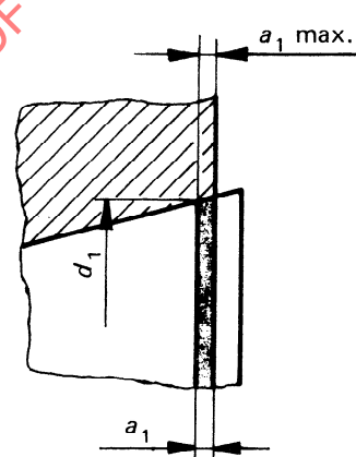
Taper plug gauge
