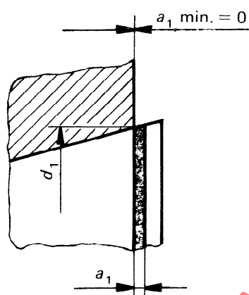
Taper plug gauge
