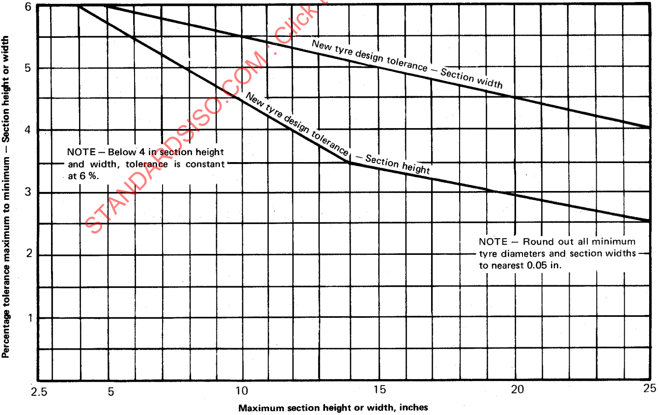
FIGURE 2 - Aircraft tyre section height and width - Dimensional tolerances (inches)
