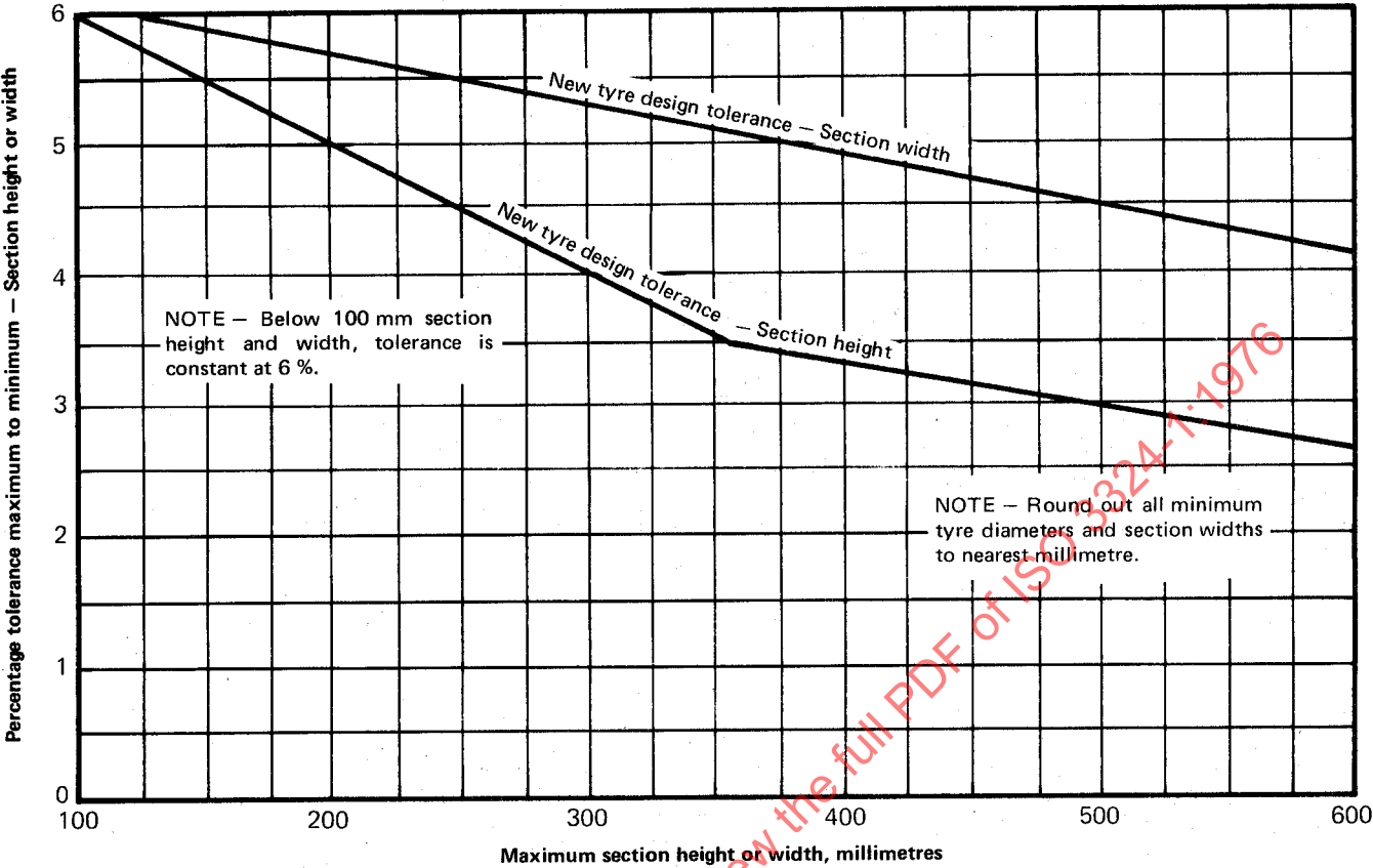
FIGURE 1 - Aircraft tyre section height and width - Dimensional tolerances (millimetres)
