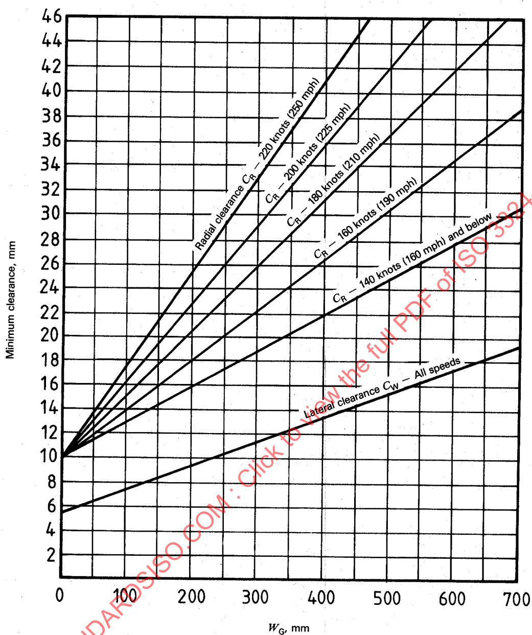
Figure 5 — Chart to be used for calculating radial C_R and lateral C_W clearances
