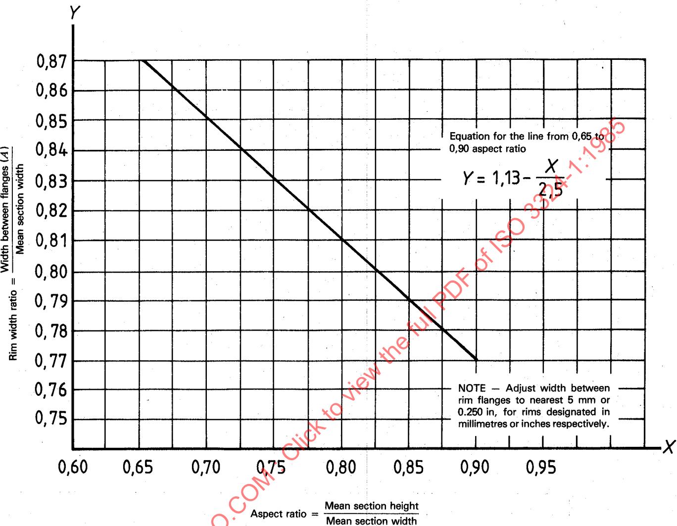
Figure 12 — Width between rim flanges (A) — Design guide
