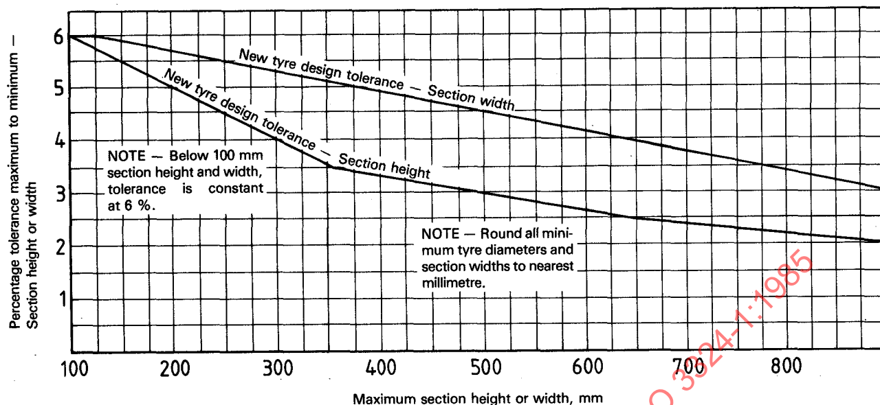
Figure 3 — New aircraft tyre section height and width — Dimensional tolerances (millimetres) 1)
