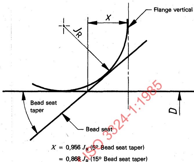
Figure 8 — Dimensioning of D specified rim diameter
