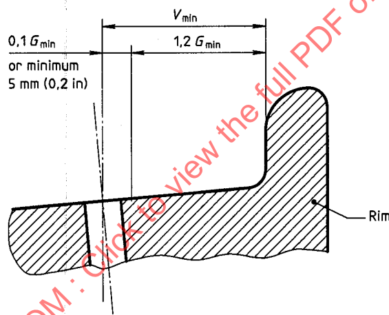
Figure 8 — Valve hole location for tube-type tyres
