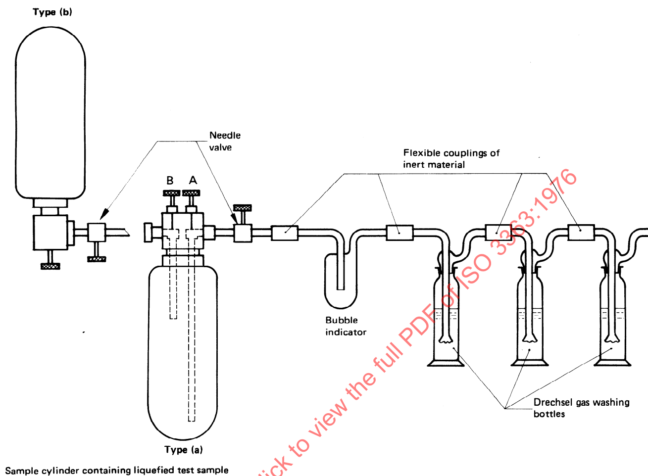
FIGURE — Apparatus for absorption of acidity for products gaseous at ordinary temperatures
