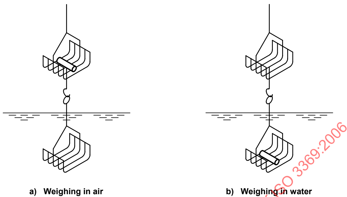
Figure 1 — Rack method
