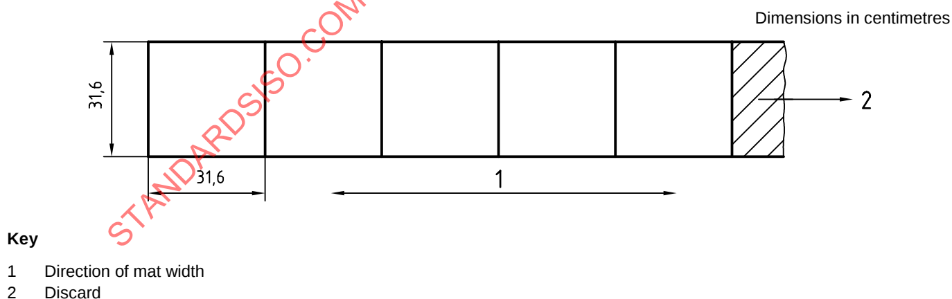
Figure 1 — Suggested method for cutting out mat specimens
