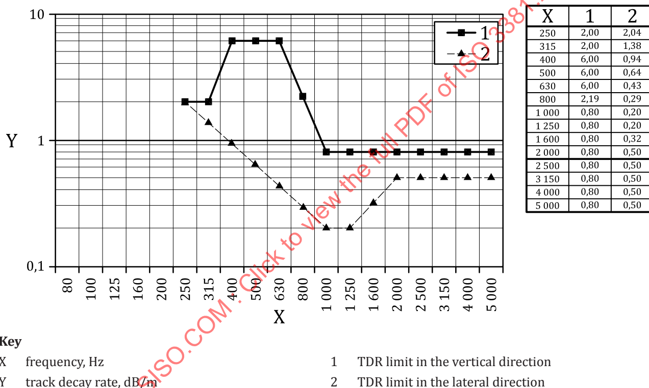
Figure C.2 — Default lower limit curves for the track decay rates
