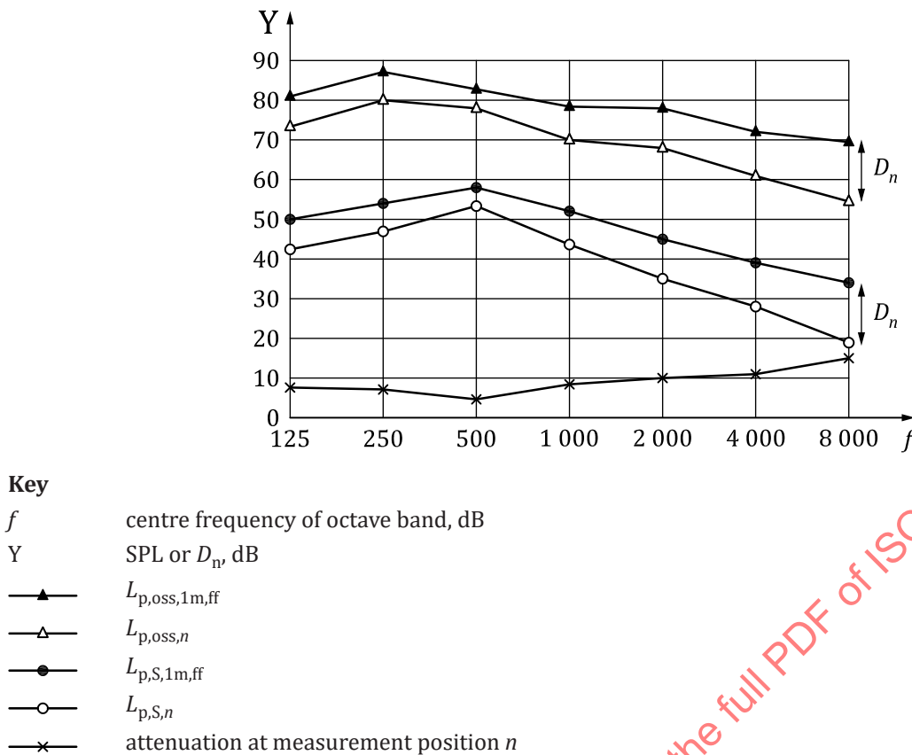
Figure 2 — Determination of the SPL of speech in measurement position n (the attenuation D_n between —▲— and —△— is the same as between —●— and —○—)
