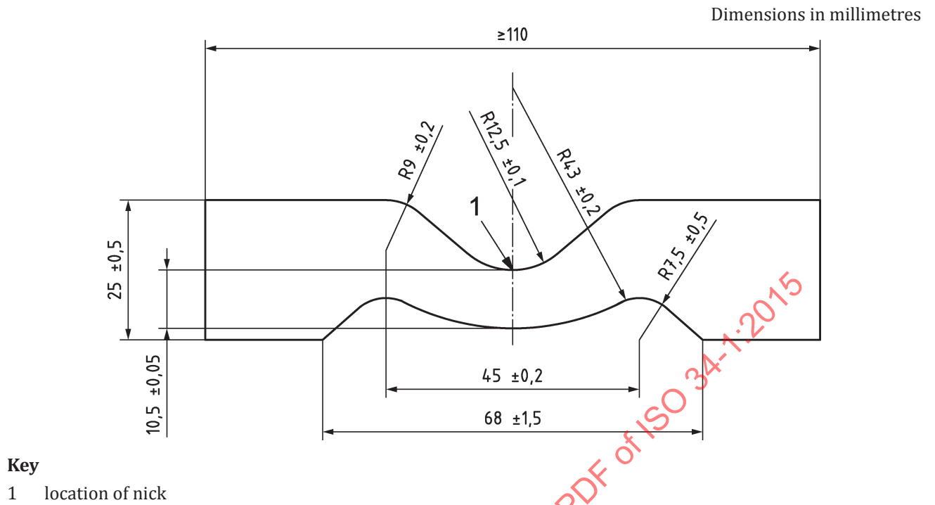
Figure 3 — Crescent test piece die
