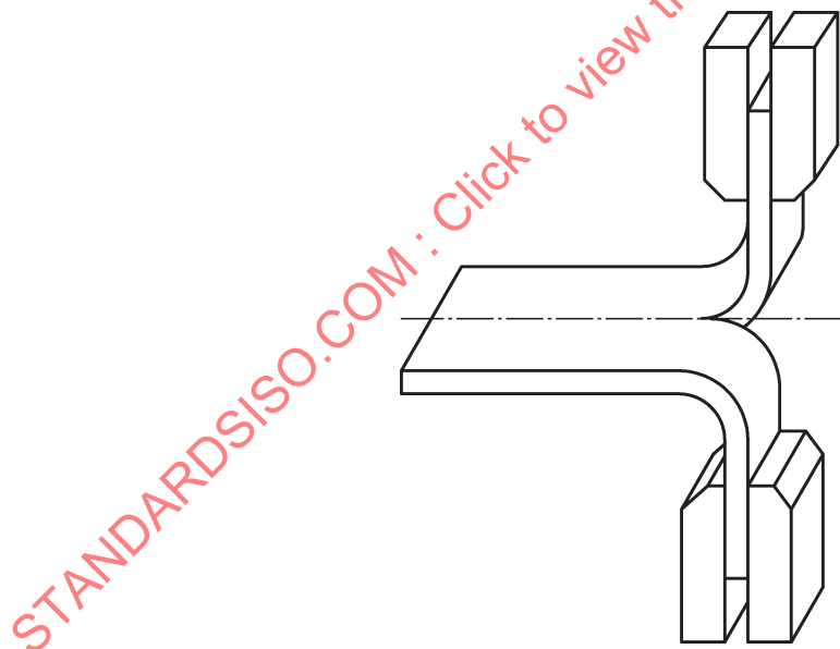
Figure 4 — Positioning of trouser test piece in testing machine
