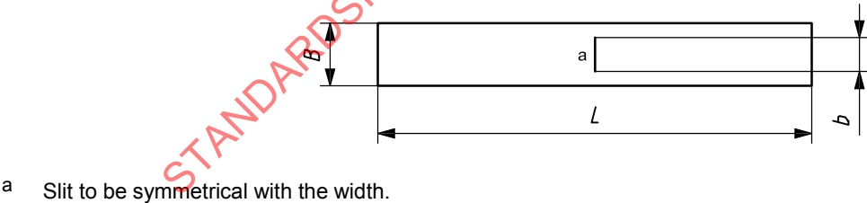
Figure 3 — Test piece
