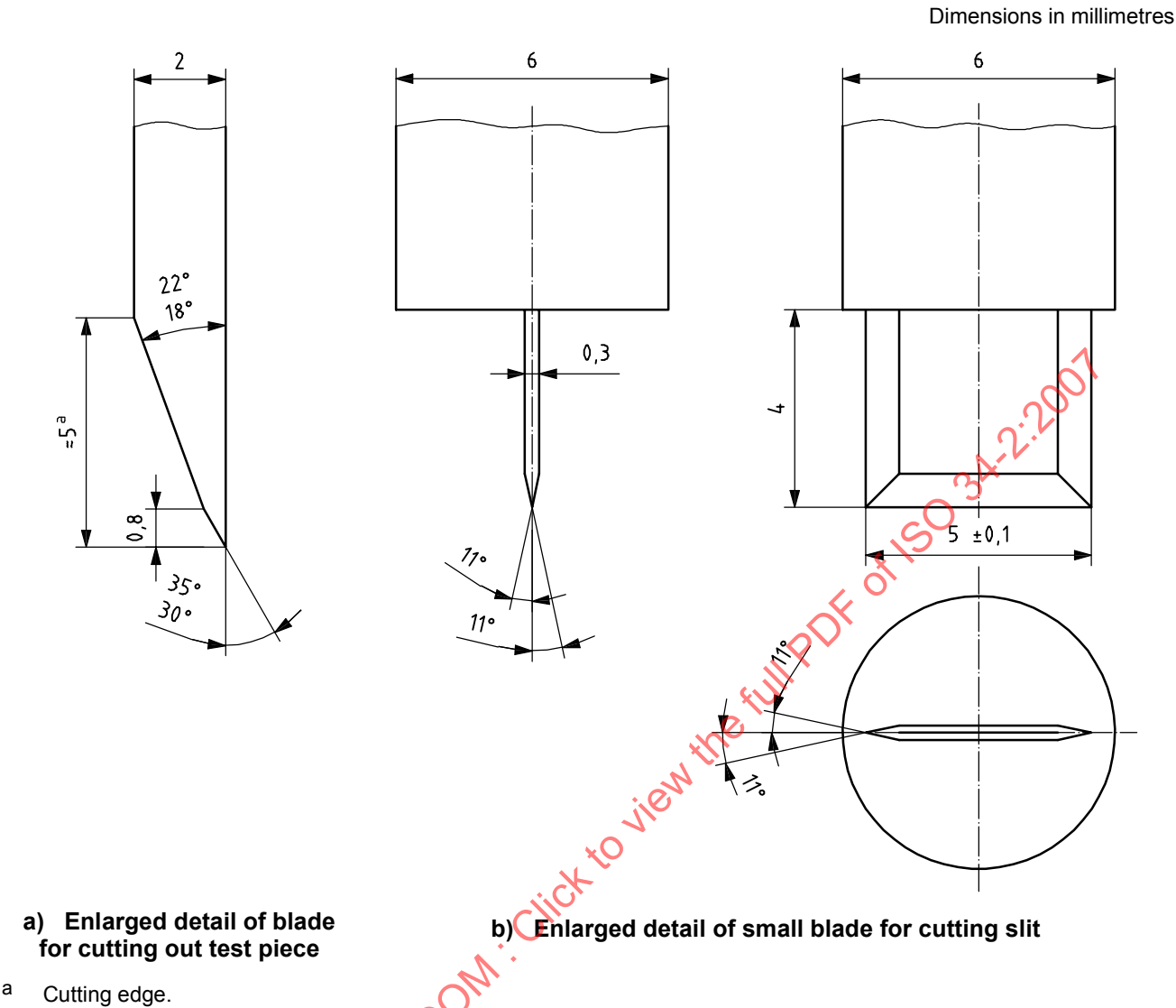
Figure 2 — Details of Delft test piece die cutting edges
