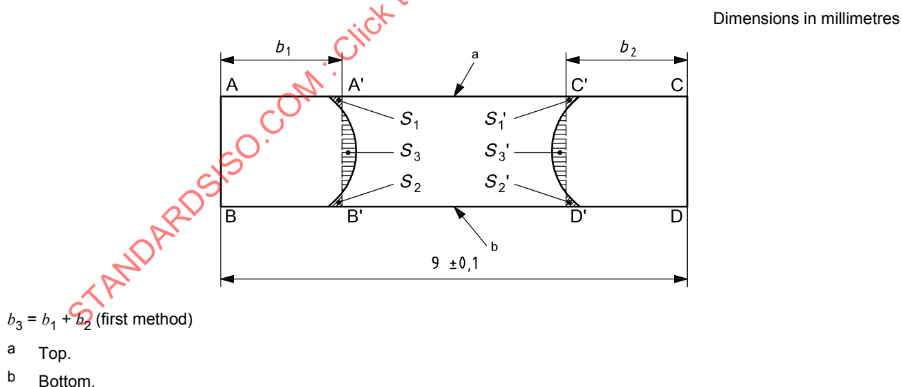
Figure 4 — Section through slit in Delft test piece
