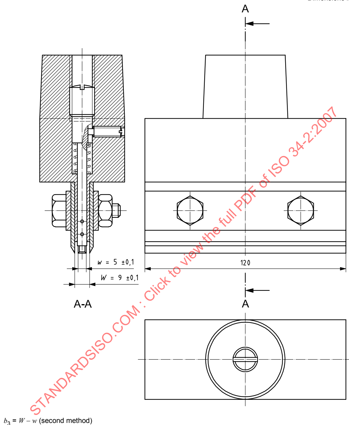
Figure 1 — Die for Delft test pieces
