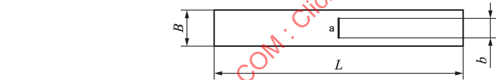
Figure 2 — Details of Delft test piece die cutting edges
