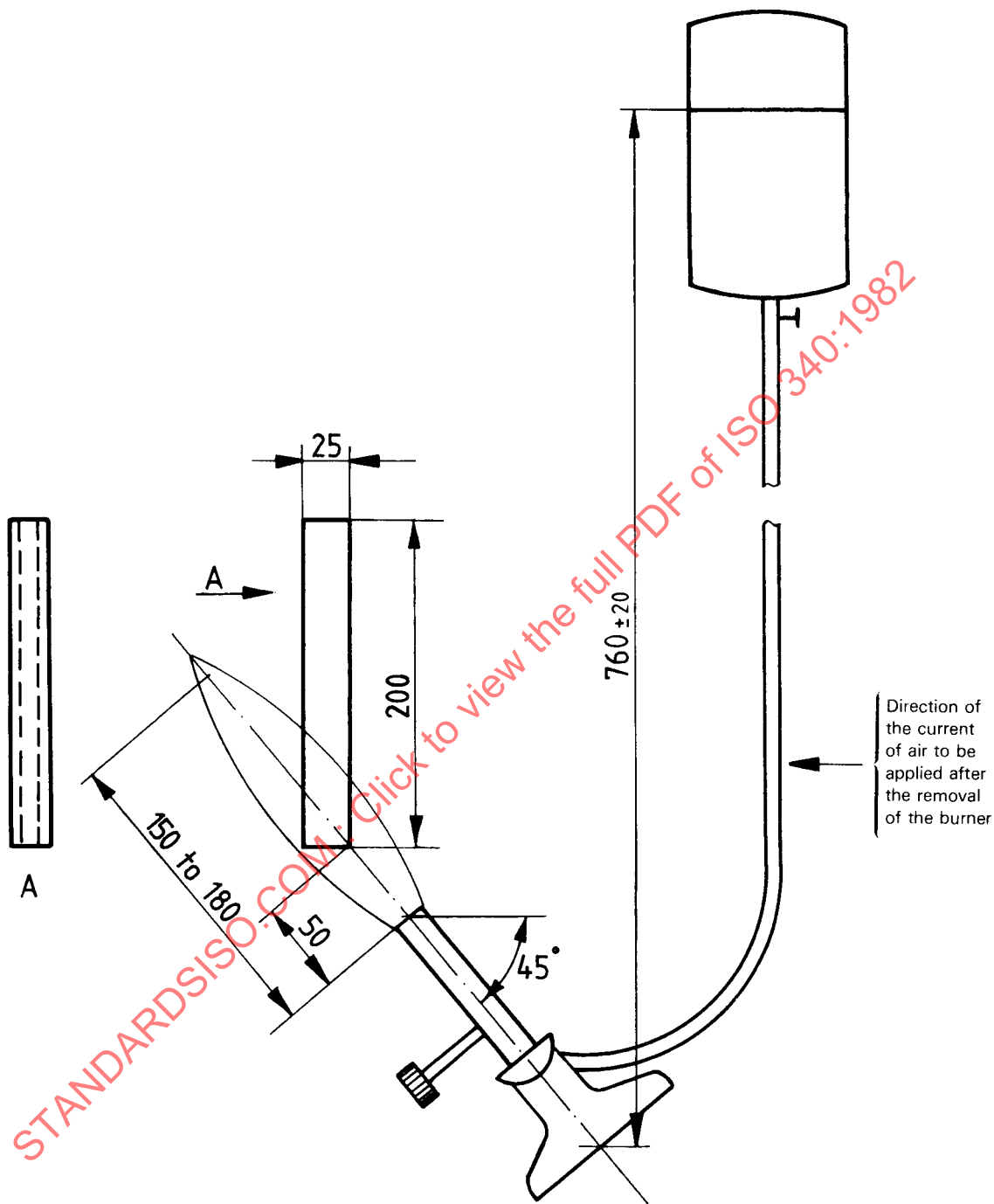
Figure 2 – Air current direction
