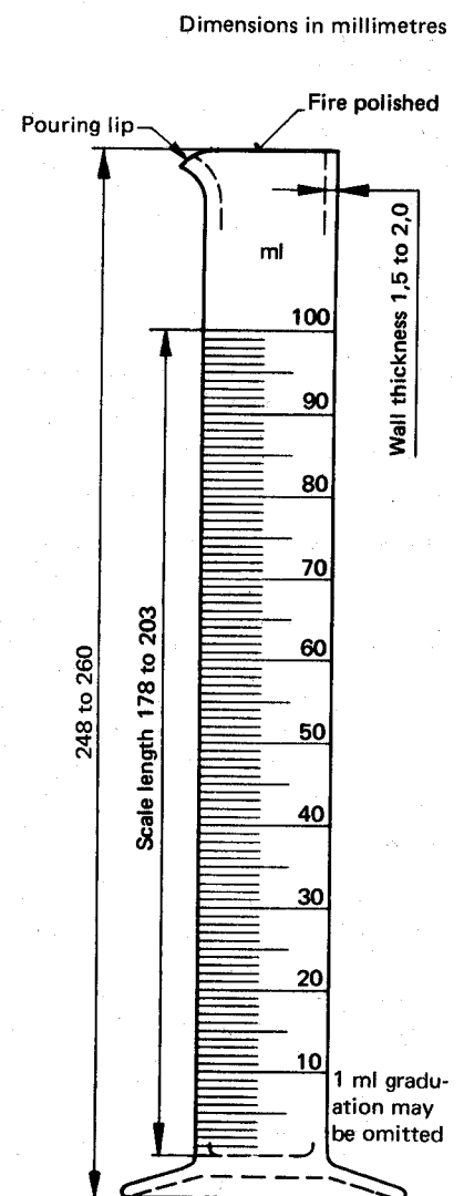
FIGURE 4 — Graduated cylinder 100 ml in 1 ml graduations Tolerance \pm 1,0 ml
