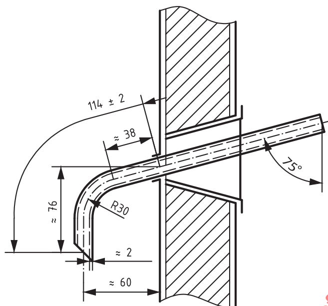
Figure 4 — Lower end of condenser tube
