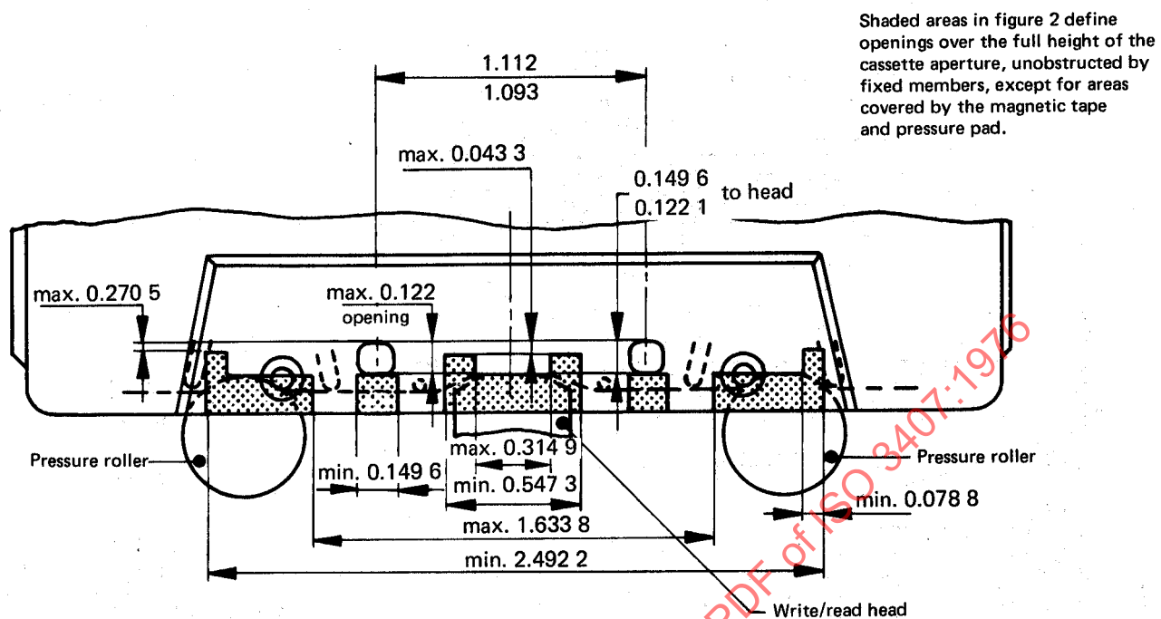
FIGURE 2b) — Position of heads — Dimensions in inches
