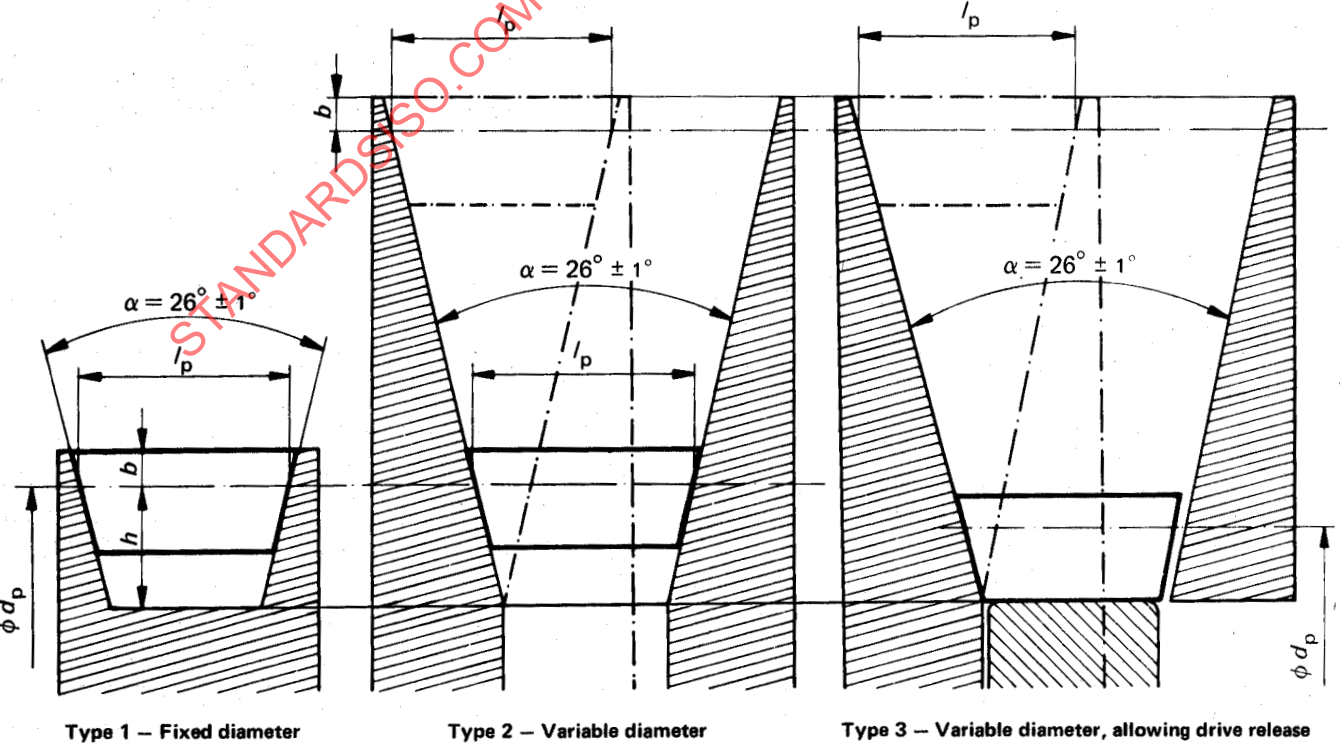
FIGURE 2 – Pulleys
