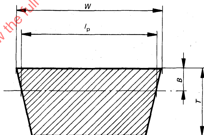
FIGURE 1 — Cross-section
