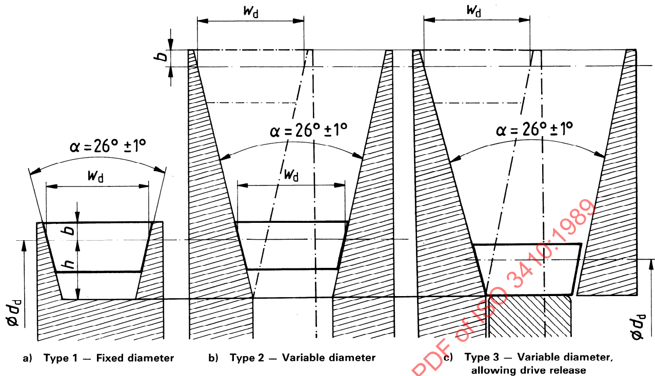
Figure 2 — Pulleys
