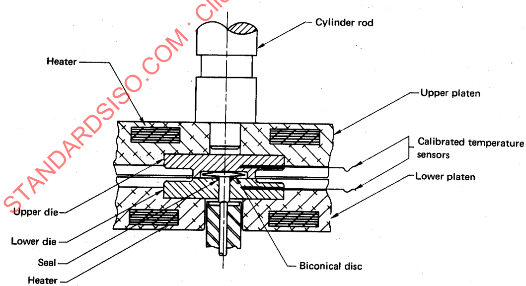
FIGURE 2 – Curemeter assembly
