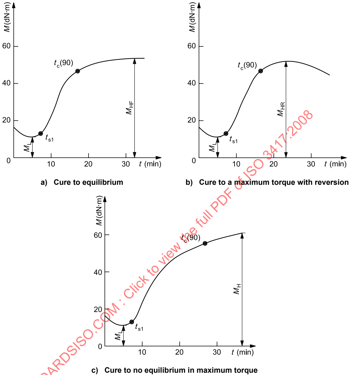
Figure 1 — Types of vulcanization curve
