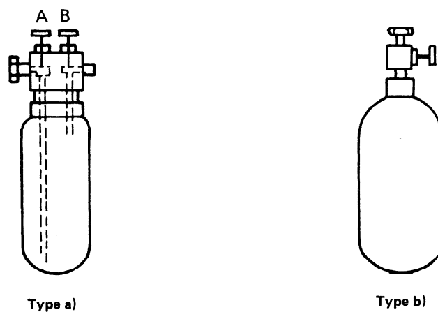
FIGURE 1 — Sample cylinder (3.1.1)
