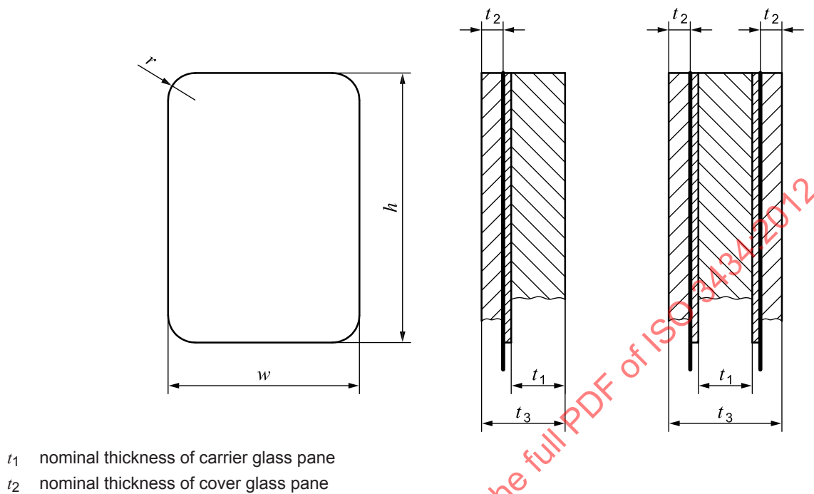
Figure 4 — Dimensions of heated glass pane
