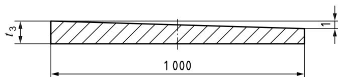
Figure 5 — Parallelism
