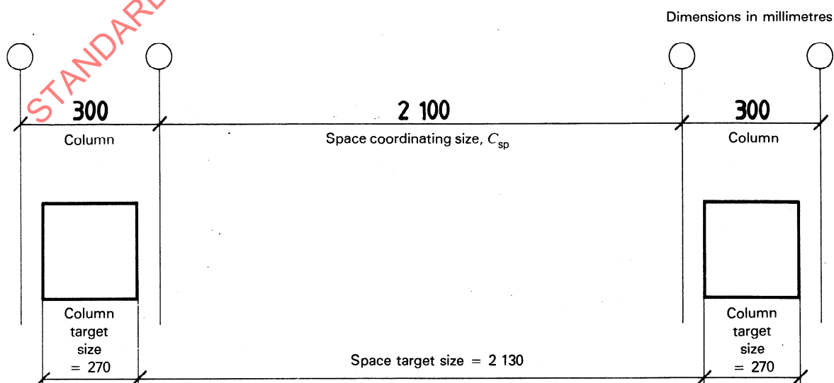
Figure 3 — Plan of opening between columns for a window
