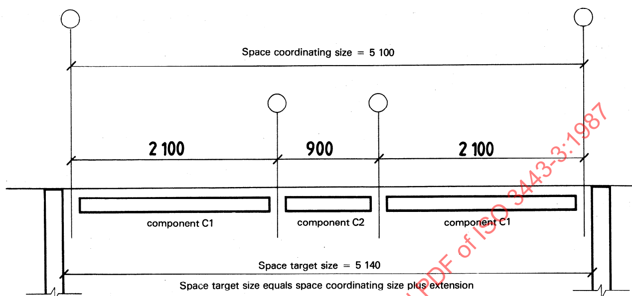
Figure 4 — Plan of opening between cross walls, for three panels
