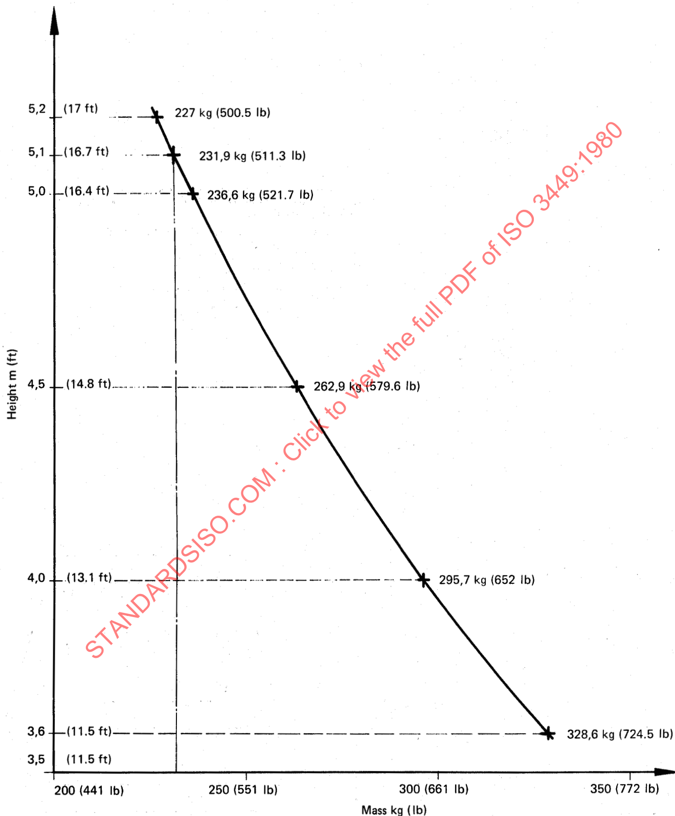
Figure 3 — Height and mass for the drop test object with the capability of developing an energy of 11 600 J (8 500 ft·lbf)
