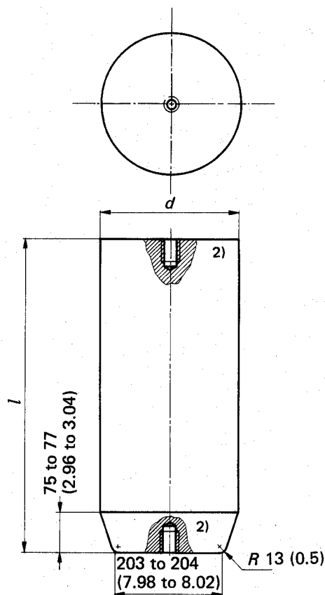
Figure 1 — Standard laboratory drop test object
