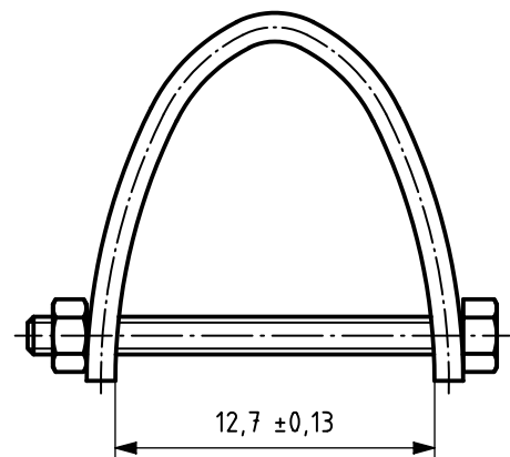
c) Stressing details (not to scale)
