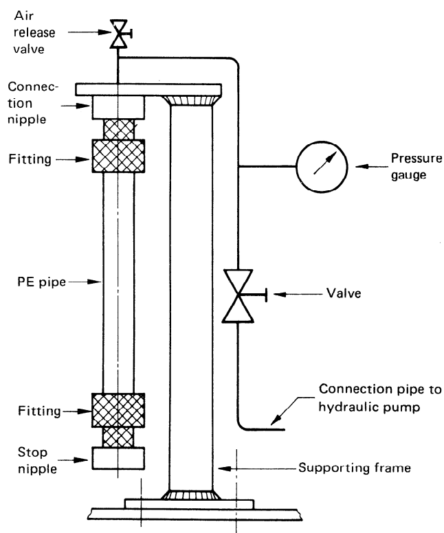
FIGURE — Diagram of suitable apparatus
