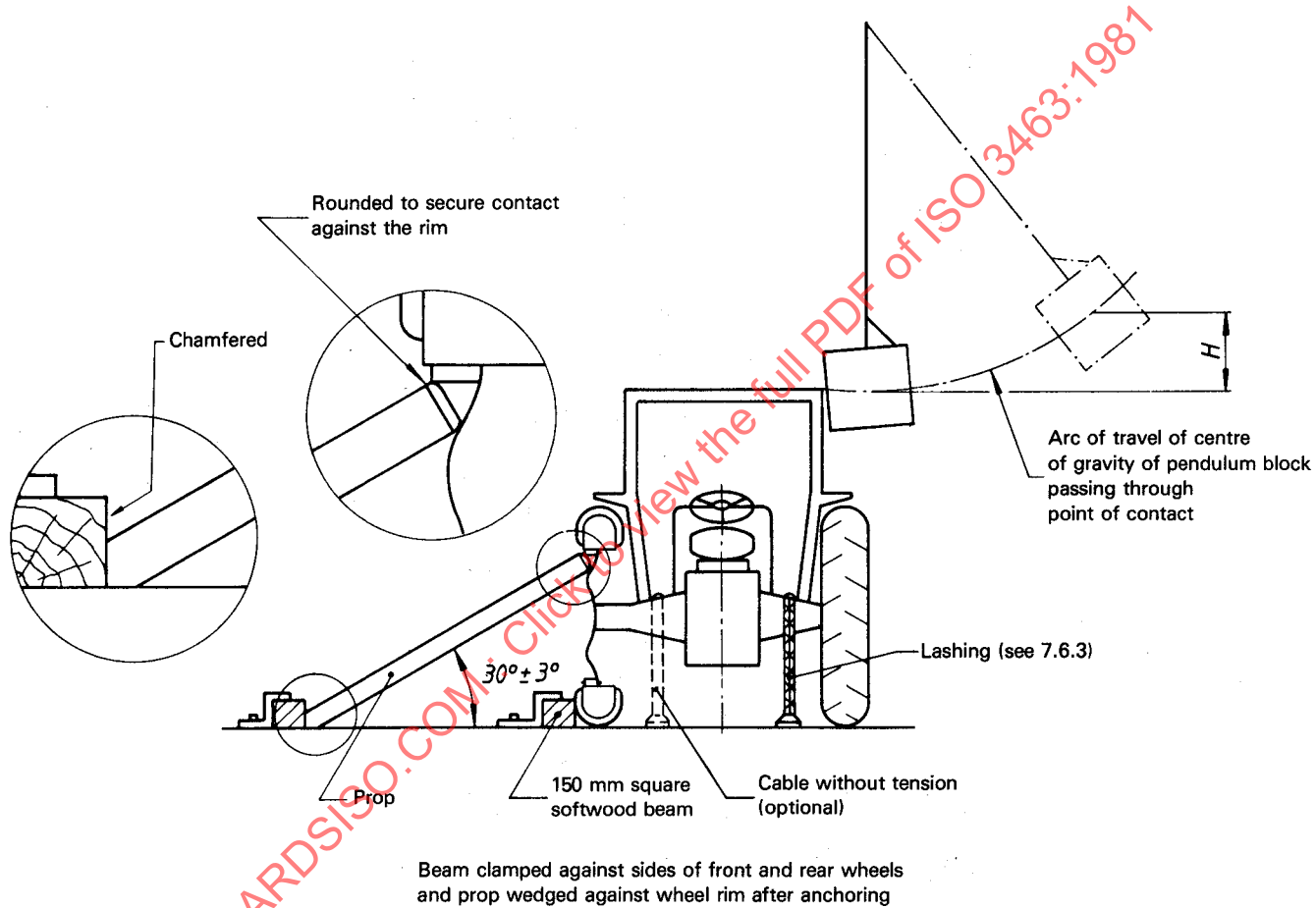
Figure 6 — Example of a method for lashing — Impact from side
