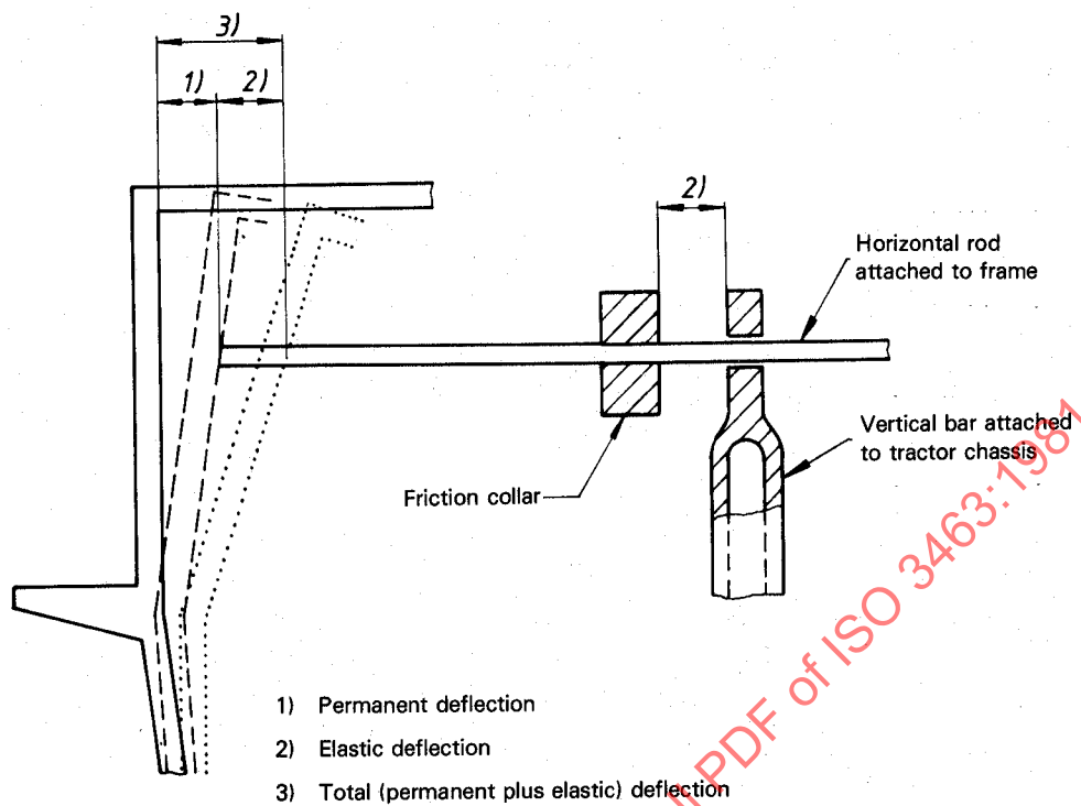
Figure 7 — Example of a device for measuring elastic deflection
