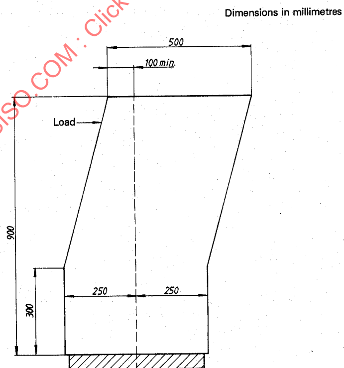
Figure 2b) — Clearance zone from the front/rear 150 mm in front of the seat reference point
