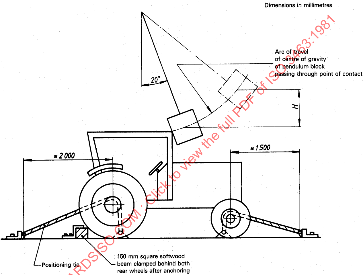
Figure 5 — Example of a method for lashing — Impact from front
