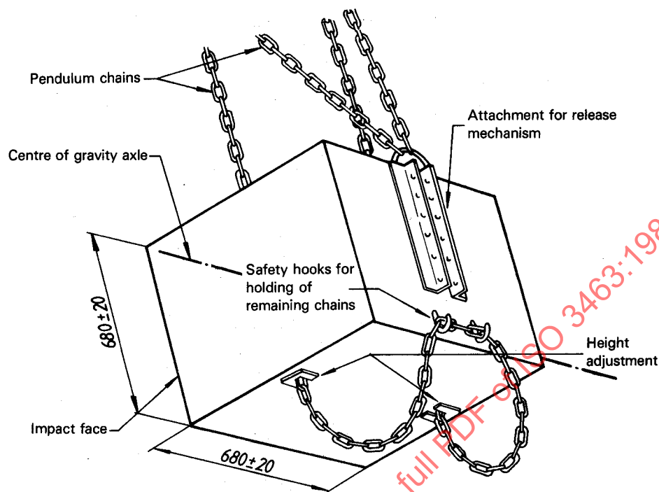
Figure 3 — Illustration of pendulum block
