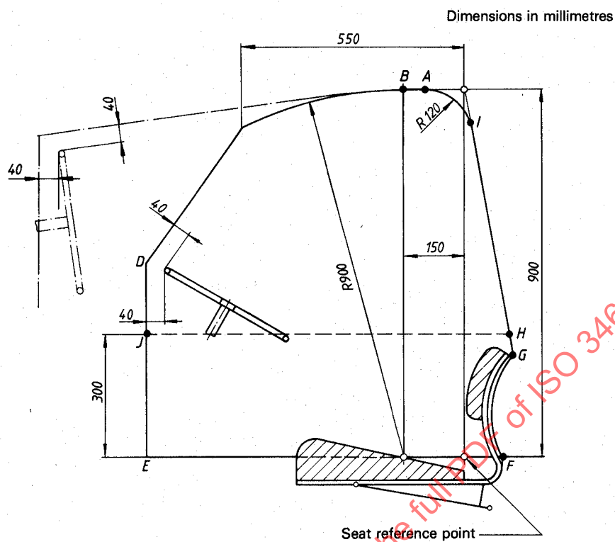
Figure 2a) — Clearance zone from the side
