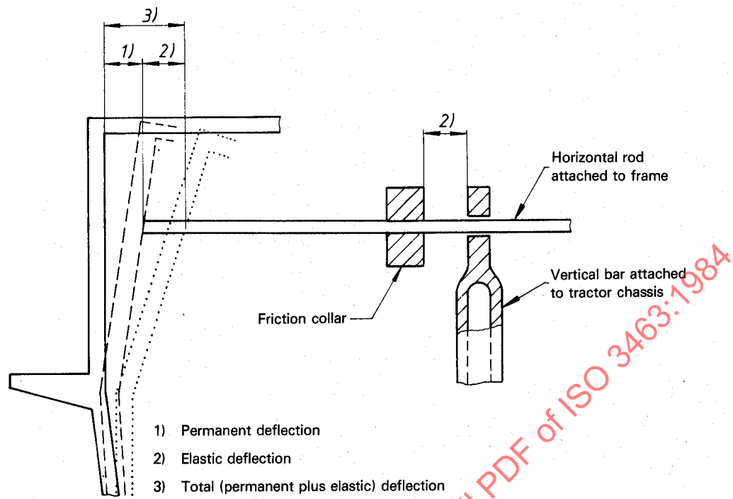
Figure 7 – Example of a device for measuring elastic deflection
