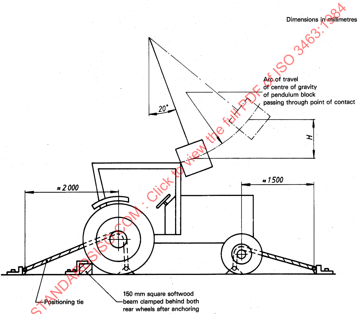
Figure 5 — Example of a method for lashing — Impact from front
