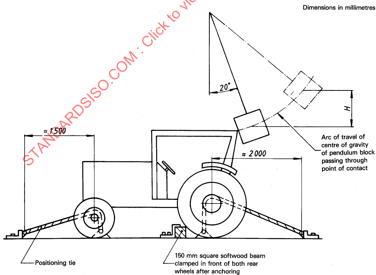
Figure 4 — Example of a method for lashing — Impact from rear
