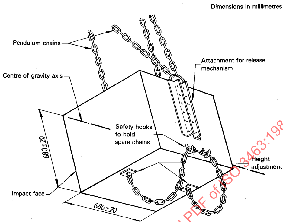
Figure 3 — Illustration of pendulum block
