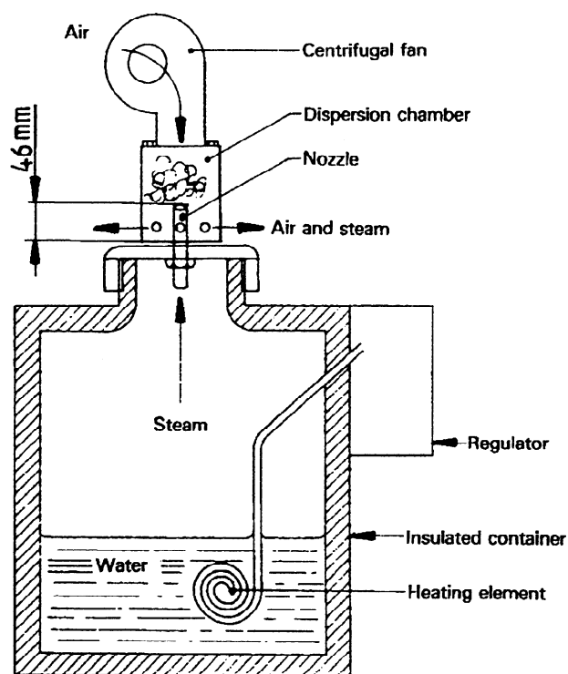
Figure 1 — Typical steam generator
