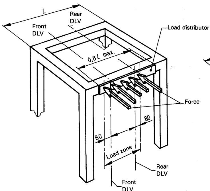
Figure 5a) — Load-distribution device for ROPS with four-post system
